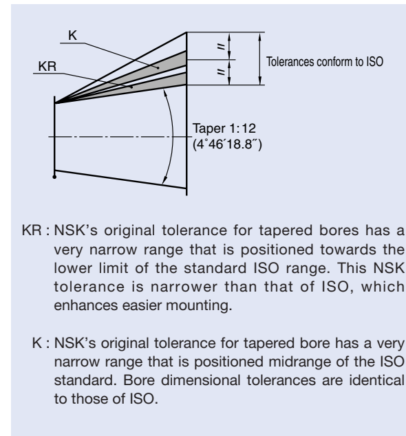
Fig. 7.2 Tolerances
