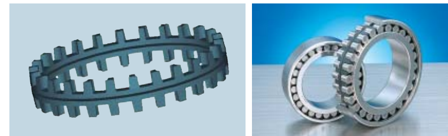
Double row CRB High Rigidity Series
